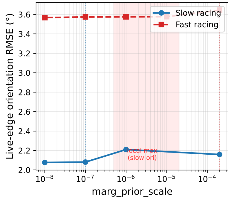
Orientation RMSE vs. prior scale
