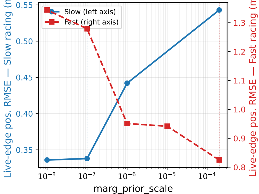
Position RMSE vs. prior scale
