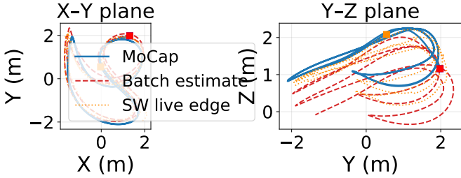
Fig. 3. Trajectory overlays (X-Y and Y-Z projections, start ■): slow racing (top) and fast racing (bottom). MoCap ground truth (solid blue), batch estimate (dashed red), SW live edge (dotted orange). Larger fast-racing deviations reflect higher dynamics ( \omega_{\text{max}} = 9.1 rad/s).
