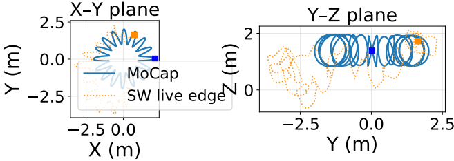
Fig. 6. backflips: MoCap ground truth (solid blue) and SW live edge (dotted orange); consistent prior, soft gate, elevation-bias correction, default RANSAC front-end). The batch estimate is omitted — at \Delta t_o=0.8 ms it is bistable (Sec. VII-B) and the SW live edge is the trustworthy result. X–Y and Y–Z projections; the vertical backflip maneuvers are visible in the Y–Z plane. Start marked ■. The estimate follows the overall donut sweep and altitude; the residual \sim 6^\circ live orientation error through flips attenuates the individual loop circles relative to ground truth.
