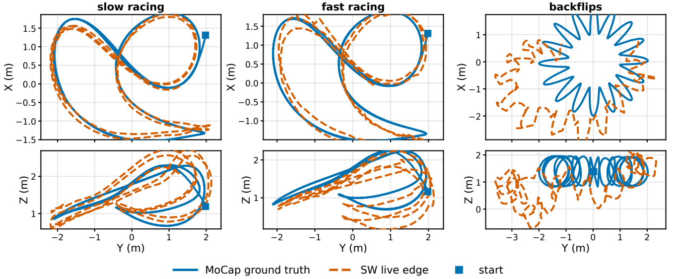
Fig. 3. Trajectory overlays for all three flights (columns): MoCap ground truth vs. the SW live edge, X-Y (top) and Y-Z (bottom) projections sharing the Y axis; start ■. Larger fast-racing deviations reflect higher dynamics ( \omega_{\max} = 9.1 rad/s); on backflips the residual \sim 6^\circ live orientation error attenuates the loop circles while the donut sweep and altitude are followed.
