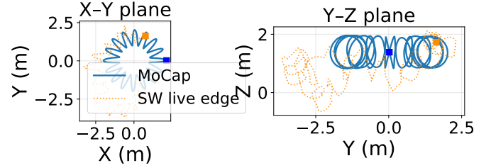
Fig. 6. backflips: MoCap ground truth (solid blue) and SW live edge (dotted orange; consistent prior, soft gate, elevation-bias correction, default RANSAC front-end). The batch estimate is omitted — at \Delta t_o=0.8 ms it is bistable (Sec. VII-B) and the SW live edge is the trustworthy result. X–Y and Y–Z projections; the vertical backflip maneuvers are visible in the Y–Z plane. Start marked \blacksquare . The estimate follows the overall donut sweep and altitude; the residual \sim 6^\circ live orientation error through flips attenuates the individual loop circles relative to ground truth.
