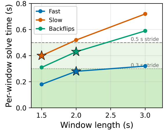
Fig. 3. [Choose this figure or Table IV.] Per-window solve time vs. window length per regime; a configuration is real-time when its solve time falls below the stride. Stars mark the per-regime real-time operating point: shrinking the window puts fast under a 0.3 s stride and slow and backflips under a 0.5 s stride, at negligible accuracy cost (Table IV). Solve times carry \sim 20\% variance.
