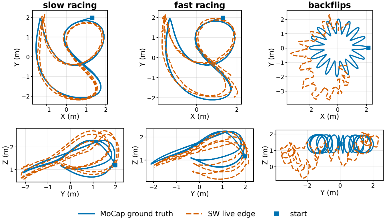
Fig. 4. Trajectory overlays for all three flights (columns): MoCap ground truth vs. the SW live edge, X-Y (top) and Y-Z (bottom) projections; start ■. Larger fast-racing deviations reflect higher dynamics ( \omega_{\max} = 9.1 \text{ rad/s} ); on backflips the residual \sim 6^\circ live orientation error attenuates the loop circles while the donut sweep and altitude are followed.
