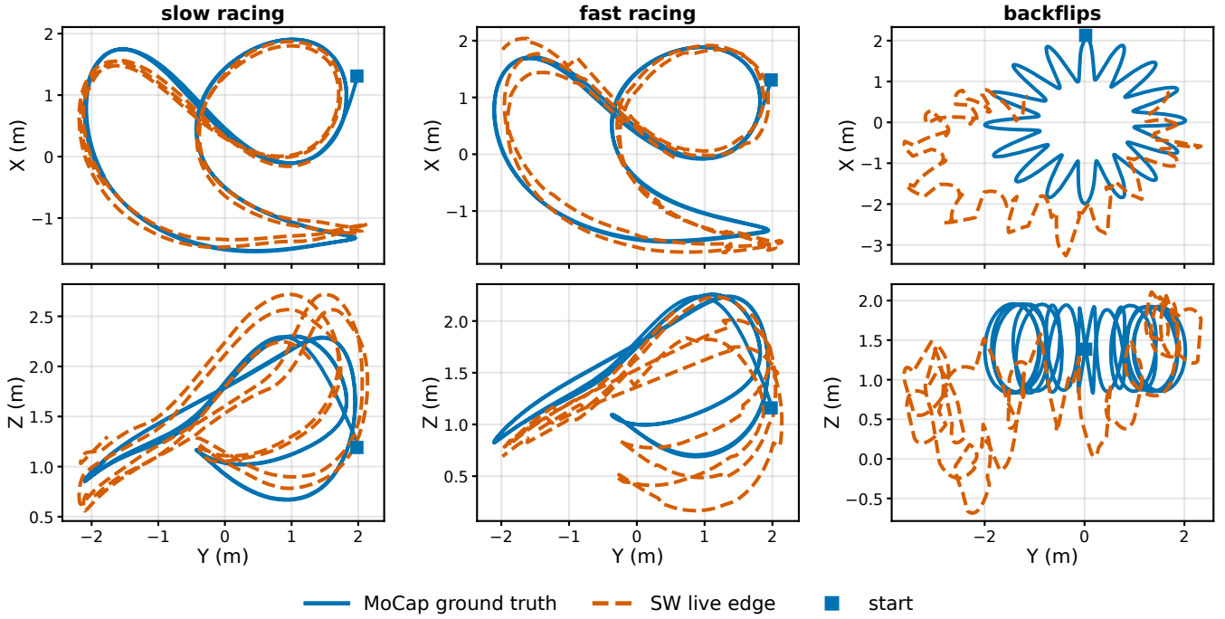
Fig. 3. Trajectory overlays for all three flights (columns): MoCap ground truth vs. the SW live edge, X-Y (top) and Y-Z (bottom) projections sharing the Y axis; start ■. Larger fast-racing deviations reflect higher dynamics ( \omega_{\max} = 9.1 rad/s); on backflips the residual \sim 6^\circ live orientation error attenuates the loop circles while the donut sweep and altitude are followed.
