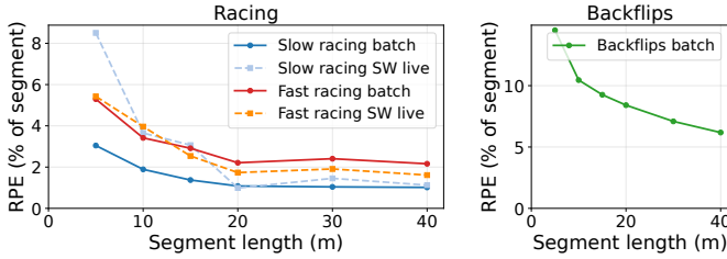
Fig. 5. KITTI-style translational RPE (end-point displacement error as % of segment length) vs. accumulated GT distance. Left: racing bags, batch (solid) and SW live edge (dashed). Right: backflips batch.
