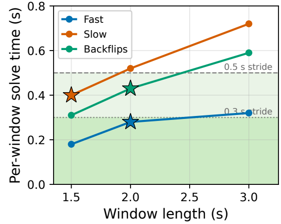
Fig. 3. [Choose this figure or Table IV.] Per-window solve time vs. window length per regime; a configuration is real-time when its solve time falls below the stride. Stars mark the per-regime real-time operating point: shrinking the window puts fast under a 0.3 s stride and slow and backflips under a 0.5 s stride, at negligible accuracy cost (Table IV). Solve times carry \sim 20\% variance.
