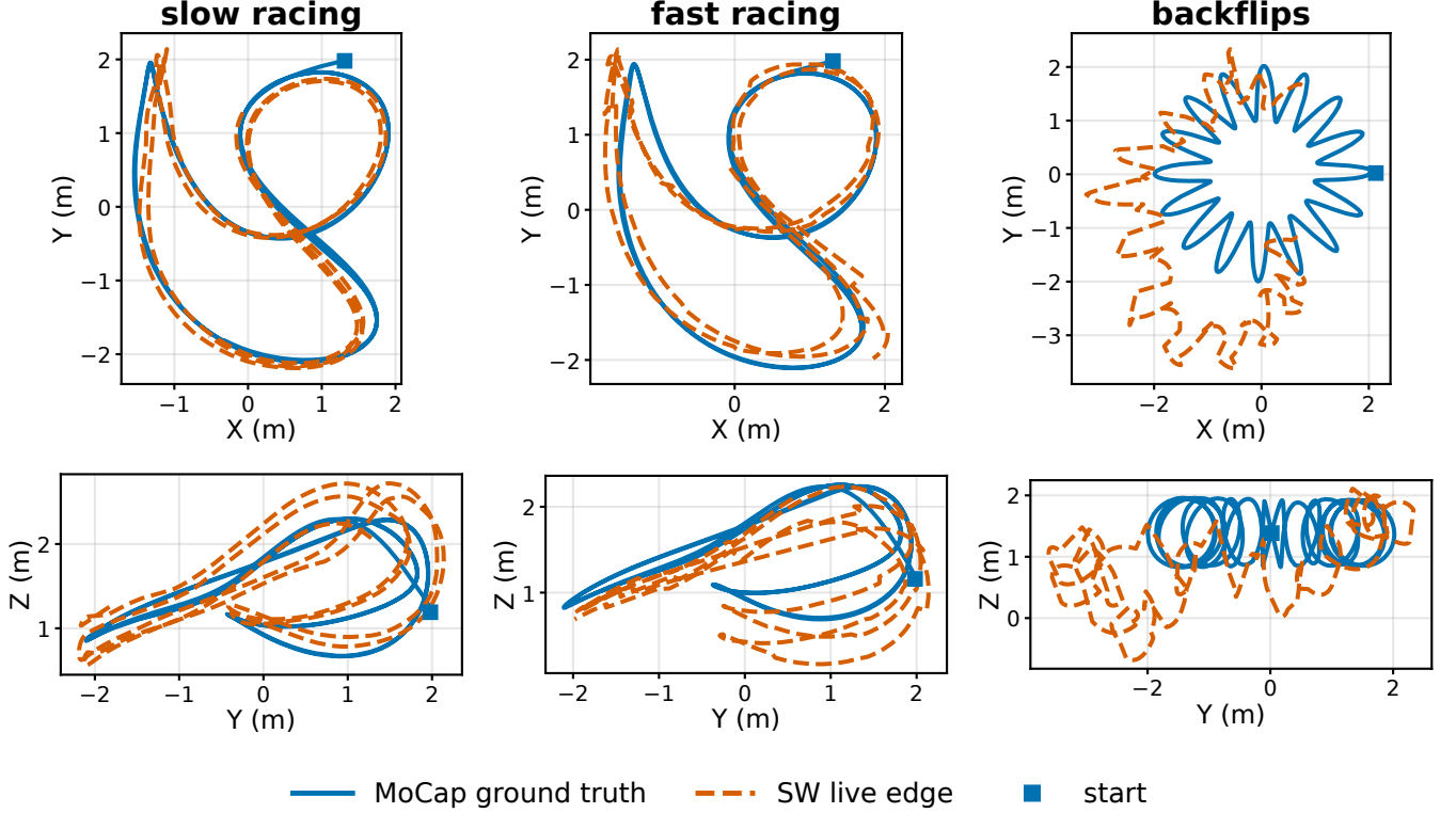
Fig. 4. Trajectory overlays for all three flights (columns): MoCap ground truth vs. the SW live edge, X-Y (top) and Y-Z (bottom) projections; start ■. Larger fast-racing deviations reflect higher dynamics ( \omega_{\max} = 9.1 \text{ rad/s} ); on backflips the residual \sim 6^\circ live orientation error attenuates the loop circles while the donut sweep and altitude are followed.
