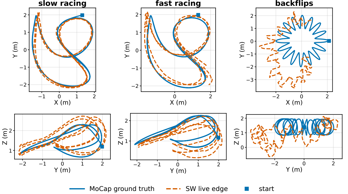
Fig. 3. Trajectory overlays for all three flights (columns): MoCap ground truth vs. the SW live edge, X-Y (top) and Y-Z (bottom) projections; start ■. Larger fast-racing deviations reflect higher dynamics ( \omega_{\max} = 9.1 \text{ rad/s} ); on backflips the residual \sim 6^\circ live orientation error attenuates the loop circles while the donut sweep and altitude are followed.
