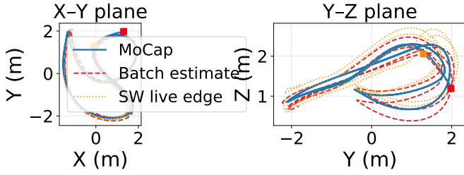
Fig. 3. slow_racing : MoCap ground truth (solid blue), batch estimate (dashed red), SW live edge (dotted orange). X-Y and Y-Z projections; start marked ■.
