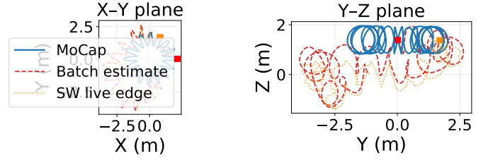
Fig. 7. backflips: MoCap ground truth (solid blue), batch estimate ( \Delta t_o = 0.8 ms, dashed red), SW live edge (consistent prior, soft gate, elevation-bias correction; dotted orange). X-Y and Y-Z projections; the vertical backflip maneuvers are visible in the Y-Z plane. Start marked \blacksquare . The estimate follows the overall donut sweep and altitude; the residual \sim 9^\circ orientation error through flips attenuates the individual loop circles relative to ground truth.
