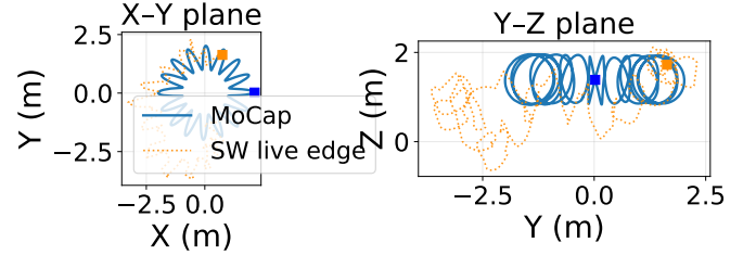
Fig. 2. backflips: MoCap ground truth (solid blue) and SW live edge (dotted orange); consistent prior, soft gate, elevation-bias correction, default RANSAC front-end). The batch estimate is omitted — at \Delta t_o=0.8\text{ms} it is bistable (Sec. VII-B) and the SW live edge is the trustworthy result. X–Y and Y–Z projections; the vertical backflip maneuvers are visible in the Y–Z plane. Start marked \blacksquare . The estimate follows the overall donut sweep and altitude; the residual \sim 6^\circ live orientation error through flips attenuates the individual loop circles relative to ground truth.
