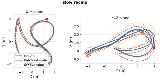
Fig. 3. slow_racing : MoCap ground truth (solid blue), batch estimate (dashed red), SW live edge (dotted orange). X-Y and Y-Z projections; start marked ■.
