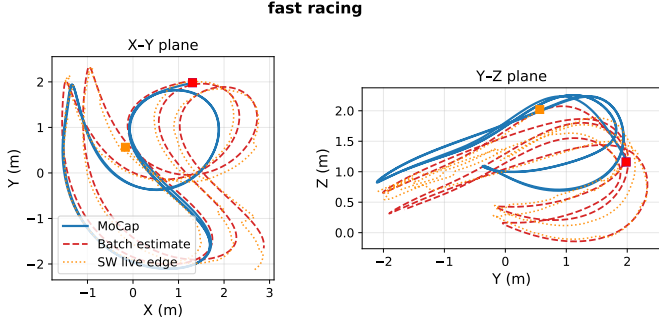
Fig. 4. fast_racing : MoCap ground truth (solid blue), batch estimate (dashed red), SW live edge (dotted orange). X-Y and Y-Z projections; start marked ■. Larger deviations reflect higher dynamics ( \omega_{\max} = 9.1 rad/s) compared to slow racing.
