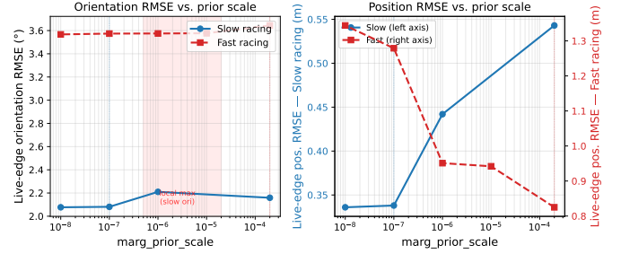
Fig. 8. Live-edge orientation (left) and position (right, dual y-axes) RMSE vs. \text{marg\_prior\_scale} . Orientation (left): slow racing shows a local maximum at 10^{-6} ; fast racing orientation is insensitive to scale. Position (right): slow racing worsens monotonically with increasing scale while fast racing improves sharply — the two bags require opposite scale regimes.
