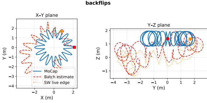
Fig. 7. backflips: MoCap ground truth (solid blue), batch estimate ( \Delta t_o=0.8 ms, dashed red), SW live edge (consistent prior, soft gate, elevation-bias correction; dotted orange). X-Y and Y-Z projections; the vertical backflip maneuvers are visible in the Y-Z plane. Start marked ■. The estimate follows the overall donut sweep and altitude; the residual \sim 9^\circ orientation error through flips attenuates the individual loop circles relative to ground truth.
