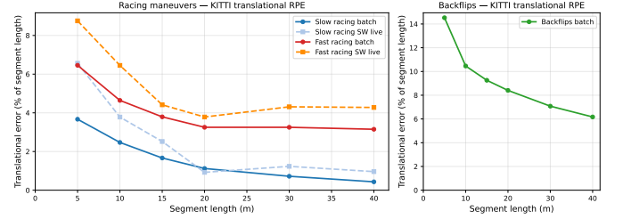
Fig. 6. KITTI-style translational RPE (end-point displacement error as % of segment length) vs. accumulated GT distance. Left: racing bags — batch (solid) and SW live edge (dashed). Right: backflips batch. Errors decrease at longer segments because the global optimizer integrates more sensor data; at short segments the 11 Hz radar provides limited constraints.
