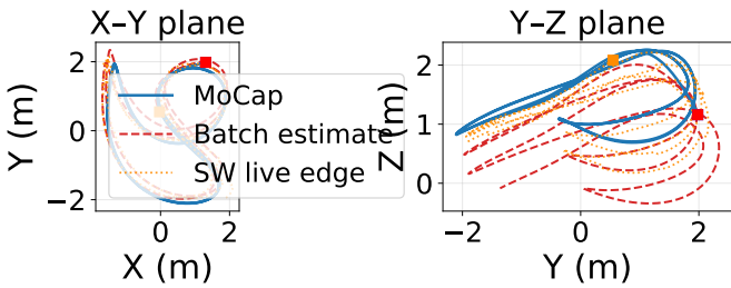
Fig. 4. fast_racing : MoCap ground truth (solid blue), batch estimate (dashed red), SW live edge (dotted orange). X-Y and Y-Z projections; start marked ■. Larger deviations reflect higher dynamics ( \omega_{\max} = 9.1 rad/s) compared to slow racing.
