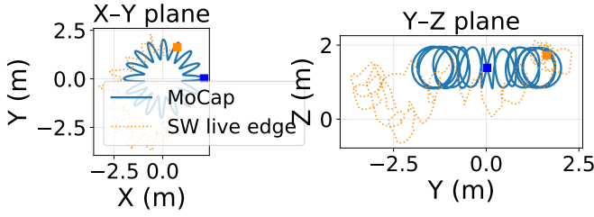
Fig. 7. backflips: MoCap ground truth (solid blue) and SW live edge (dotted orange; consistent prior, soft gate, elevation-bias correction, default RANSAC front-end). The batch estimate is omitted — at \Delta t_o=0.8 ms it is bistable (Sec. VII-B) and the SW live edge is the trustworthy result. X-Y and Y-Z projections; the vertical backflip maneuvers are visible in the Y-Z plane. Start marked ■. The estimate follows the overall donut sweep and altitude; the residual \sim 6^\circ live orientation error through flips attenuates the individual loop circles relative to ground truth.
