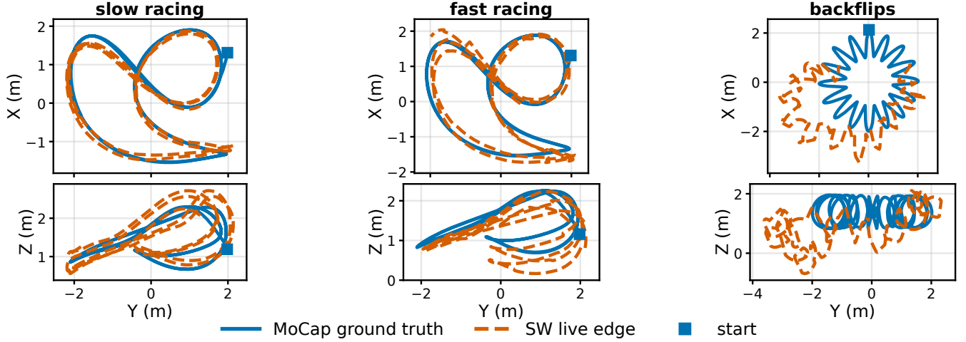
Fig. 2. Trajectory overlays for all three flights (columns): MoCap ground truth vs. the SW live edge, X–Y (top) and Y–Z (bottom) projections sharing the Y axis; start ■. Larger fast-racing deviations reflect higher dynamics ( \omega_{\max} = 9.1 rad/s); on backflips the residual \sim 6^\circ live orientation error attenuates the loop circles while the donut sweep and altitude are followed.
