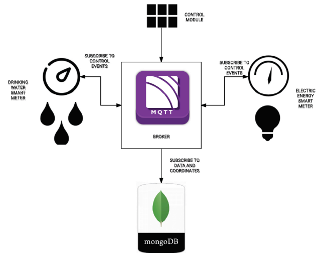
Figure 5: MQTT Broker
