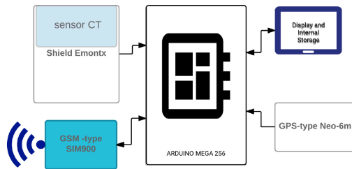
Figure 4: Electric Energy Smart Meter
