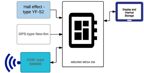
Figure 3: Water Smart Meter
