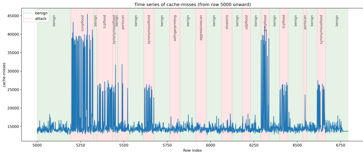
Figure 9: cache-misses timeline
