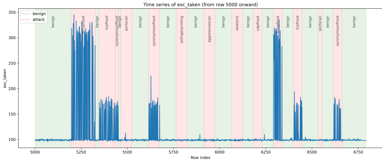
Figure 10: exc-taken timeline
