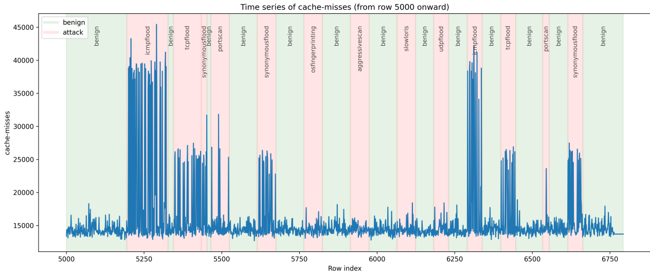
Figure 9: cache-misses timeline
