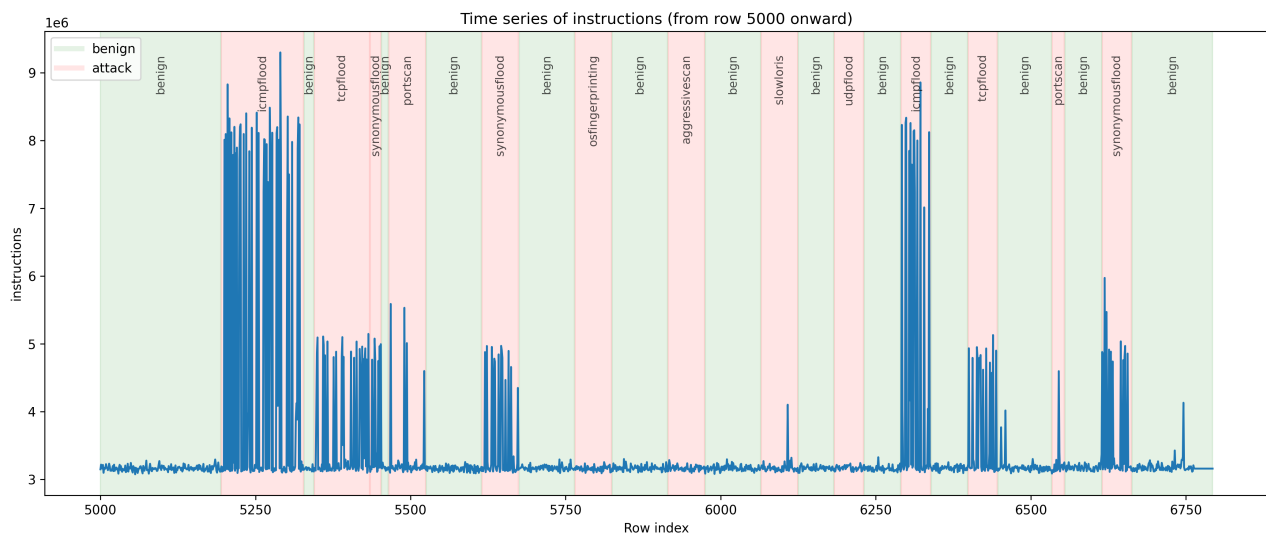
Figure 11: instructions timeline
