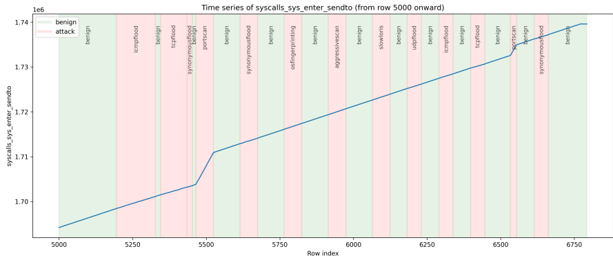
Figure 27: syscalls_sys_enter_sendto timeline
