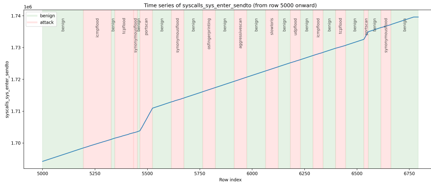
Figure 27: syscalls_sys_enter_sendto timeline
