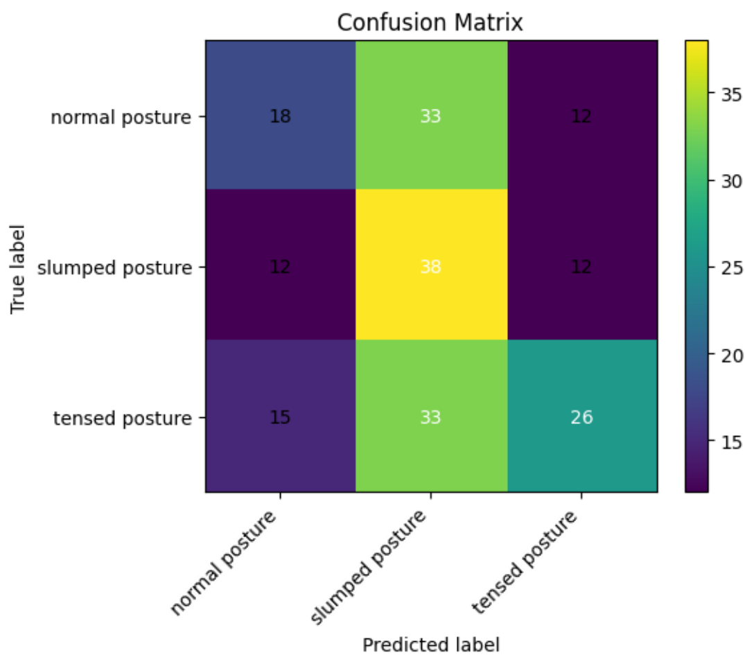
Figure 11: Confusion matrix showing again preference of ‘slumped posture’ class.
