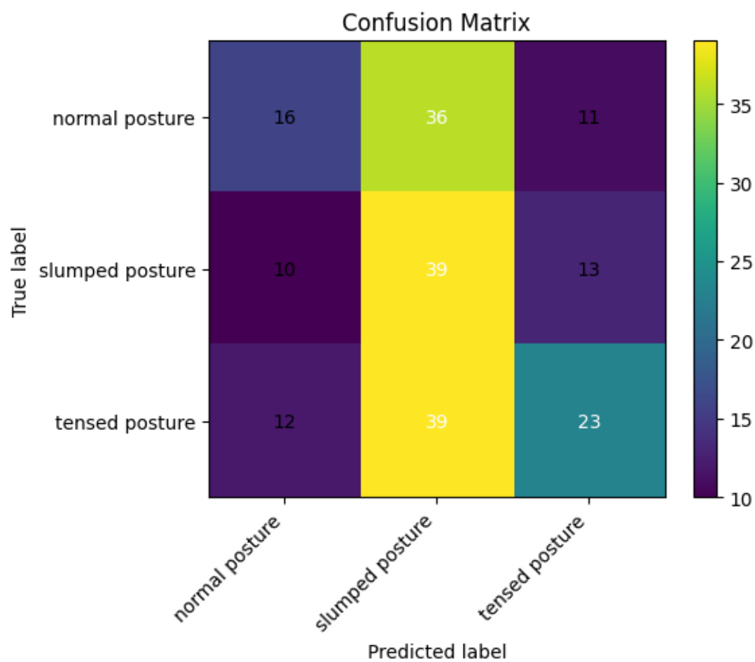
Figure 10: Confusion matrix showing preference of 'slumped posture' class.
