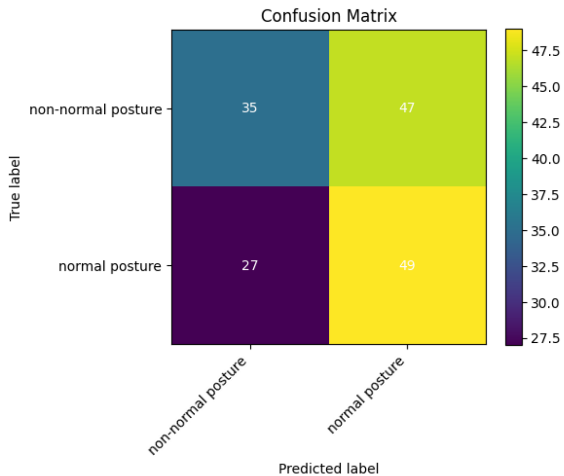
Figure 6: Confusion matrix showing 'normal posture' class preference.
