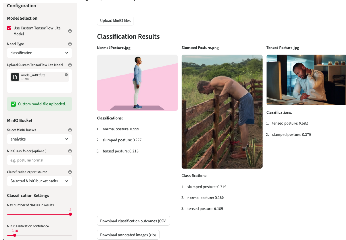
Figure 3: Streamlit Web App with classification of postures using the build quantized model from Training 4 (Table 15).
