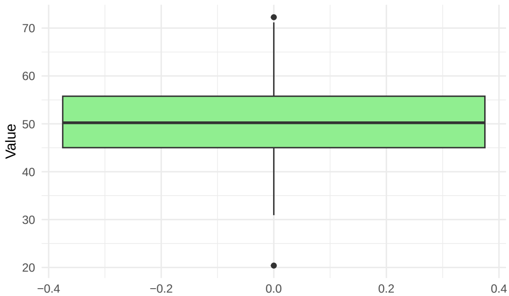
Box Plot
