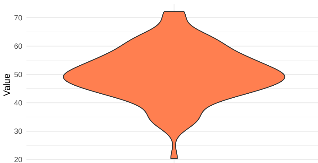
Violin Plot
