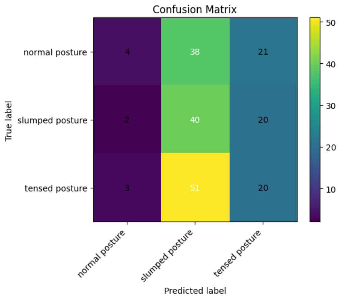
Figure 7: 3-Class - Training 2
