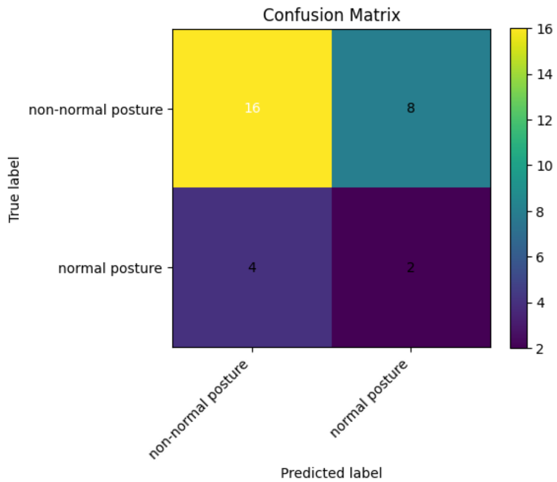
Figure 3: 2-Class - Training 1
