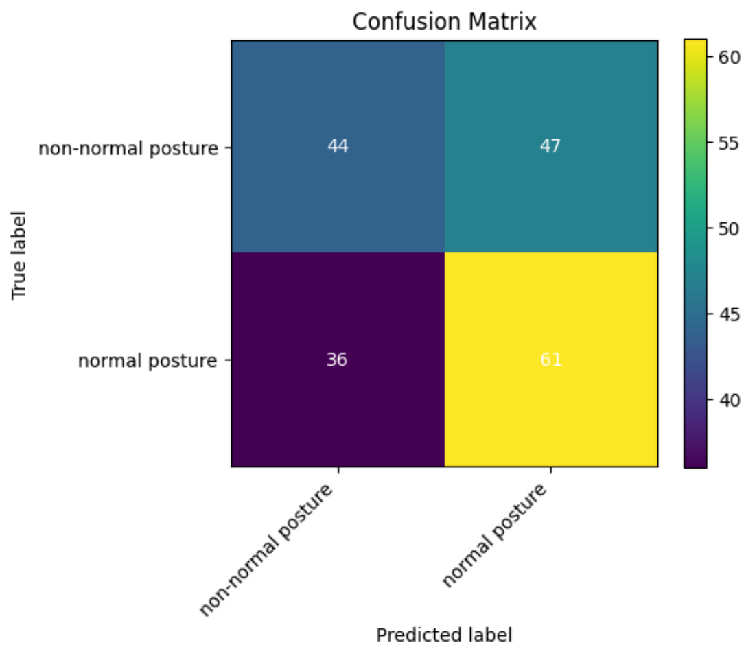
Figure 5: 2-Class - Training 3
