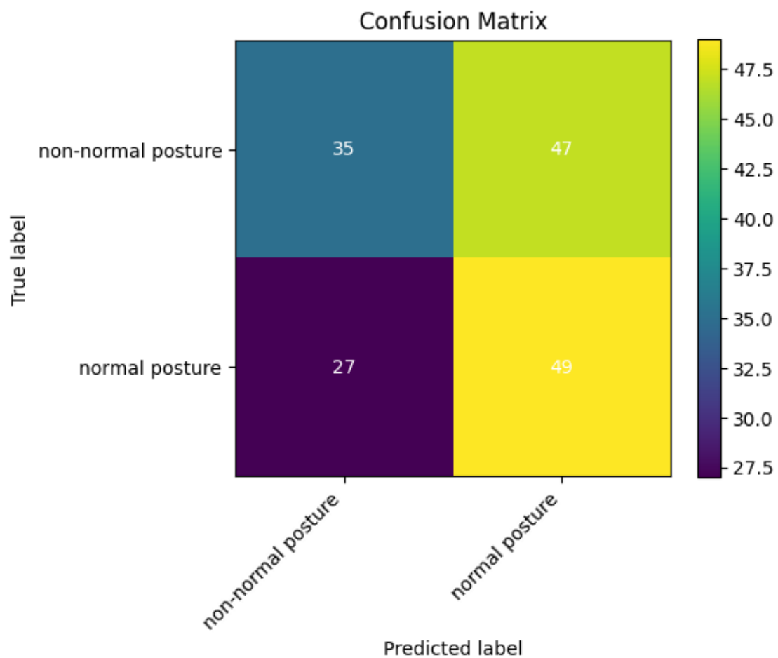
Figure 4: 2-Class - Training 2
