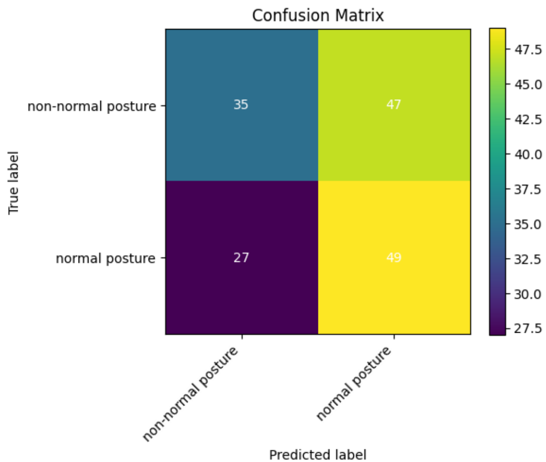
Figure 6: Figure 6: Confusion matrix showing 'normal posture' class preference.
