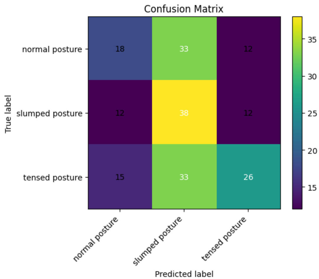
Figure 11: Figure 11: Confusion matrix showing again preference of 'slumped posture' class.
