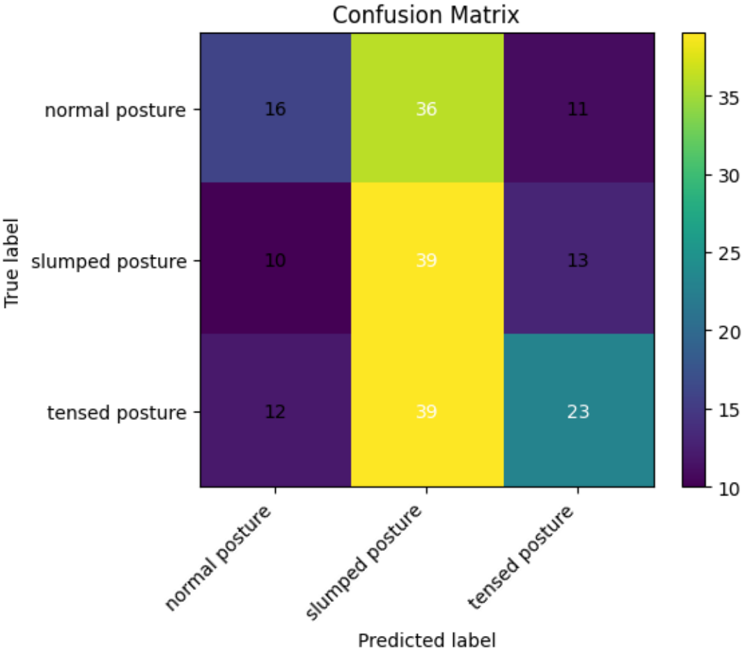
Figure 10: Figure 10: Confusion matrix showing preference of ‘slumped posture’ class.
