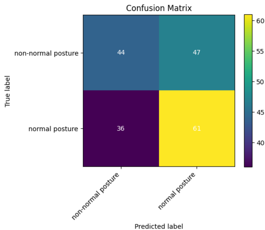
Figure 7: Figure 7: Confusion matrix again showing ‘normal posture’ class preference.
