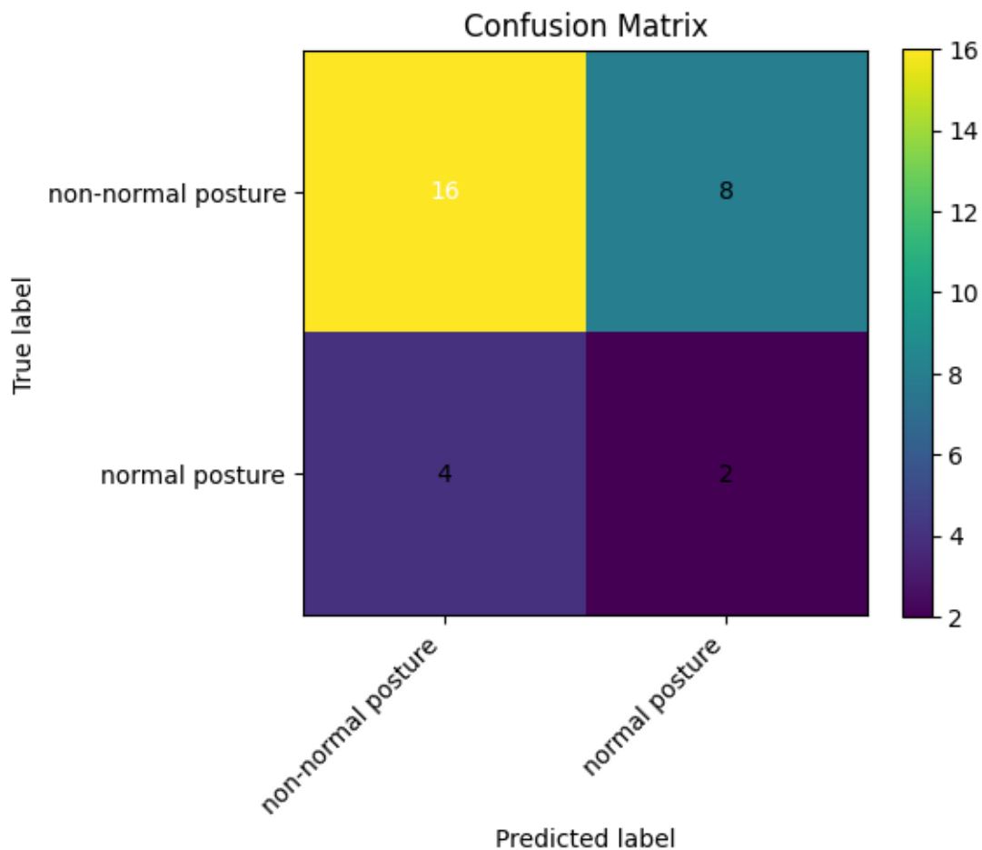
Figure 5: Figure 5: Confusion matrix showing low amount of test images and preference for category ‘non-normal posture’.
