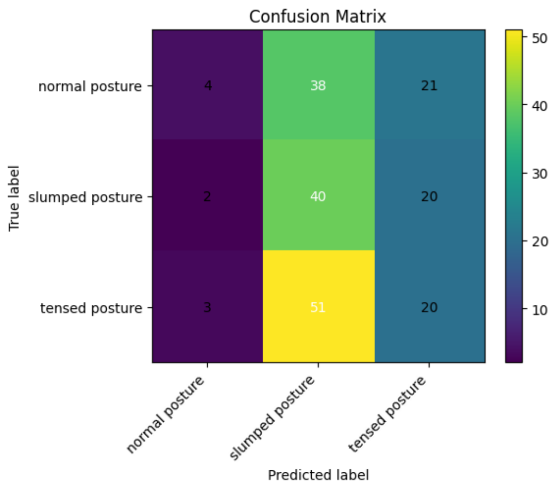
Figure 9: Figure 9: Confusion matrix showing under-representation of 'normal posture' class and a preference for 'slumped posture'.
