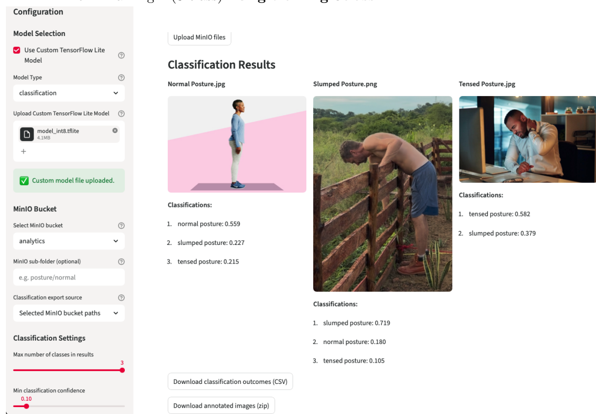
Figure 3: Streamlit Web App with classification of postures using the build quantized model from Training 4 (3-class) ?@fig-training-3class-4.
