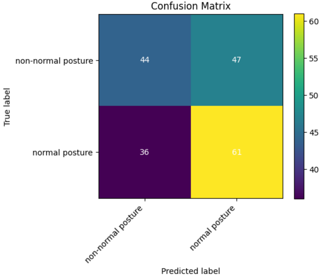
Figure 5: 2-Class - Training 3
