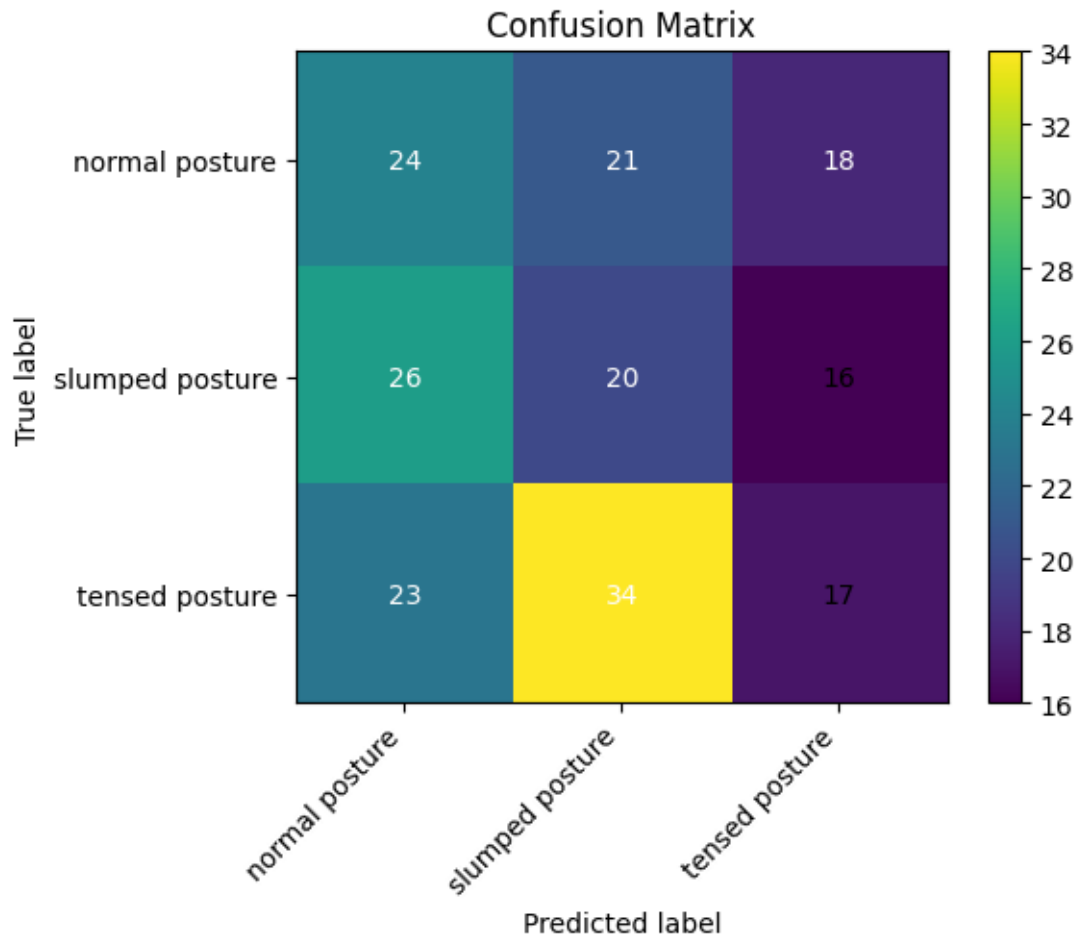
Figure 6: 3-Class - Training 4
