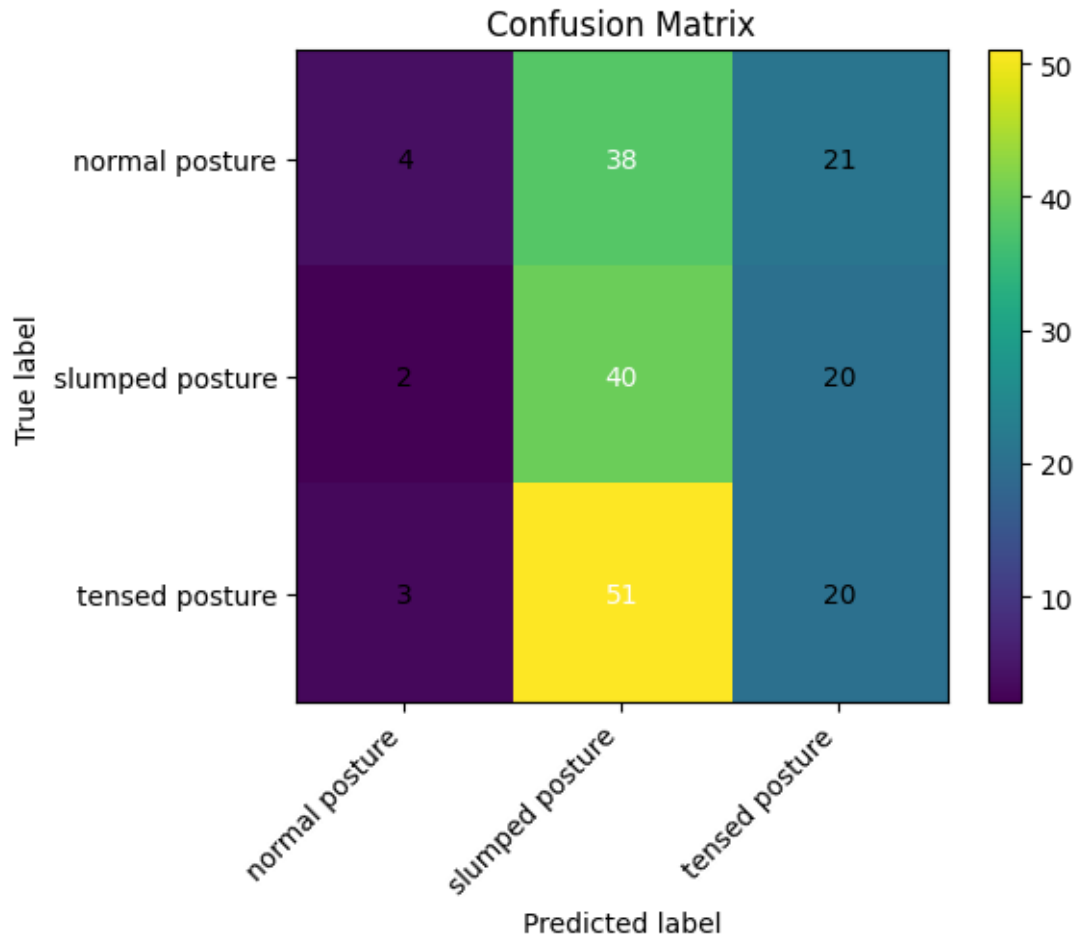
Figure 2: Training 1
