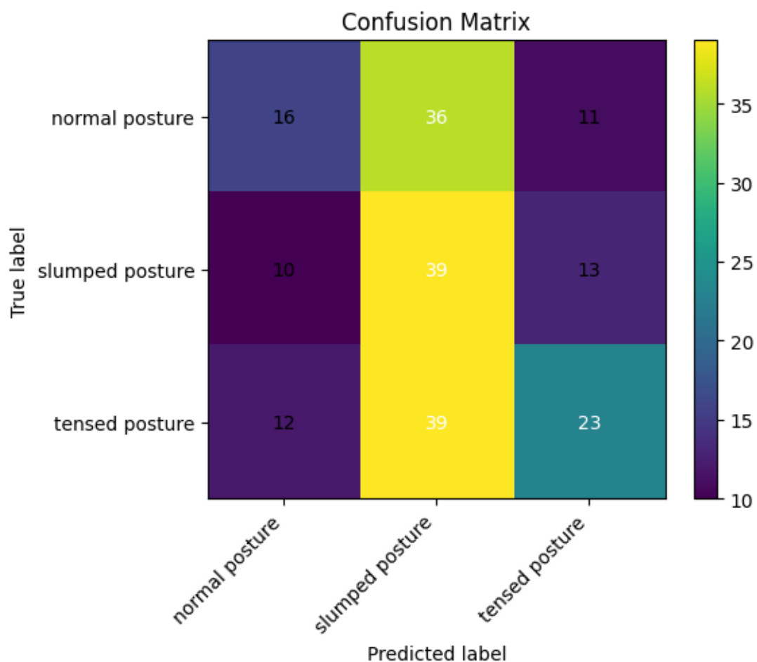
Figure 3: Training 2
