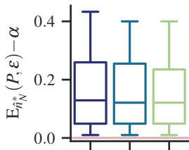
Overpessimistic
