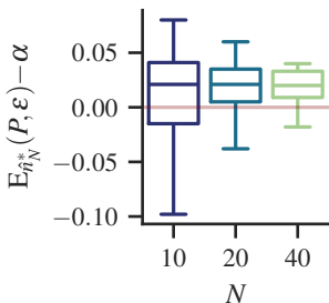
Bootstrap
