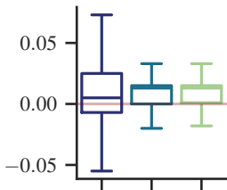
Permutation
