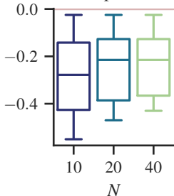
Overoptimistic
