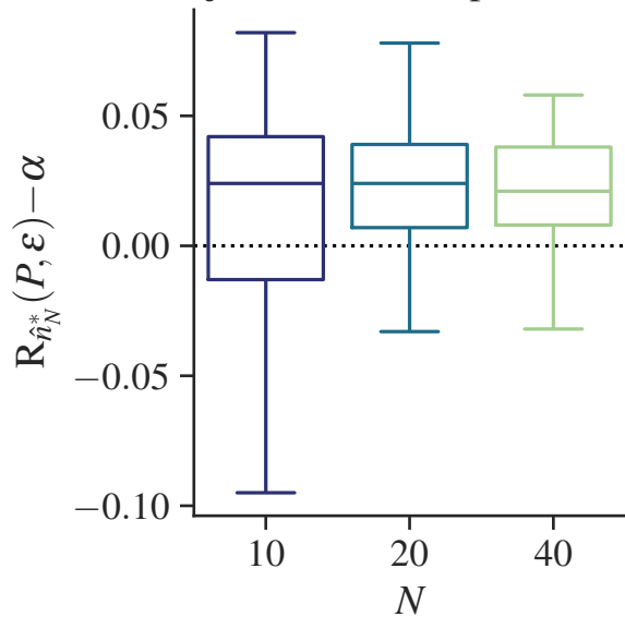
disjoint = False, replace=True
