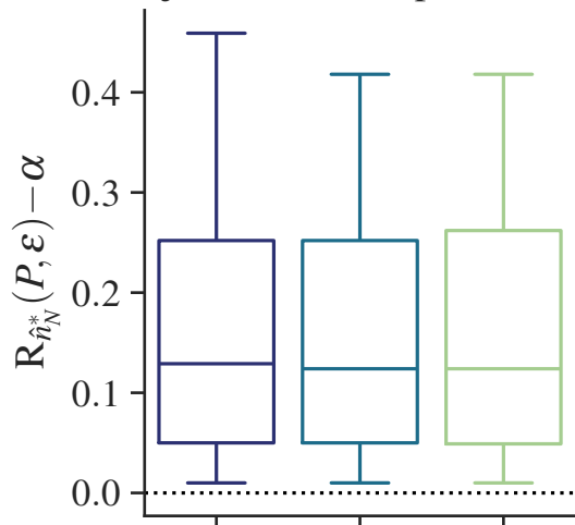
disjoint = True, replace=True
