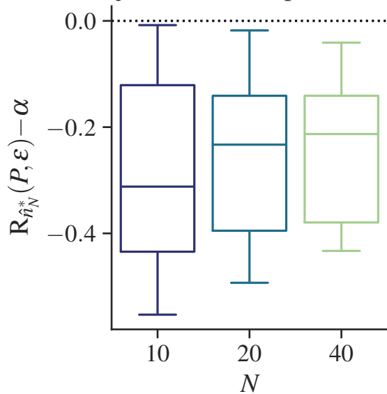
disjoint = False, replace=False
