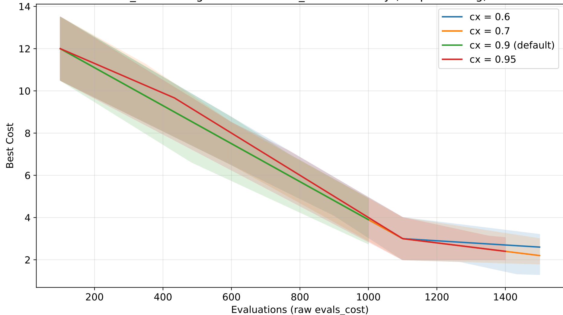
GA_GC convergence - crossover_rate sensitivity (GraphColoring)
