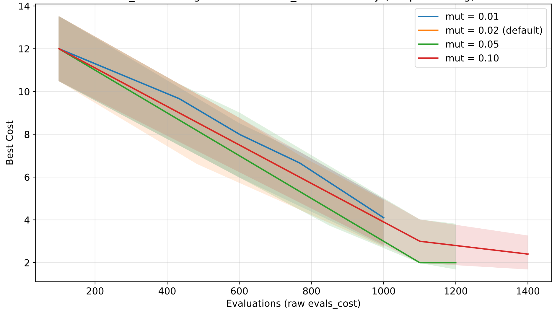
GA_GC convergence - mutation_rate sensitivity (GraphColoring)
