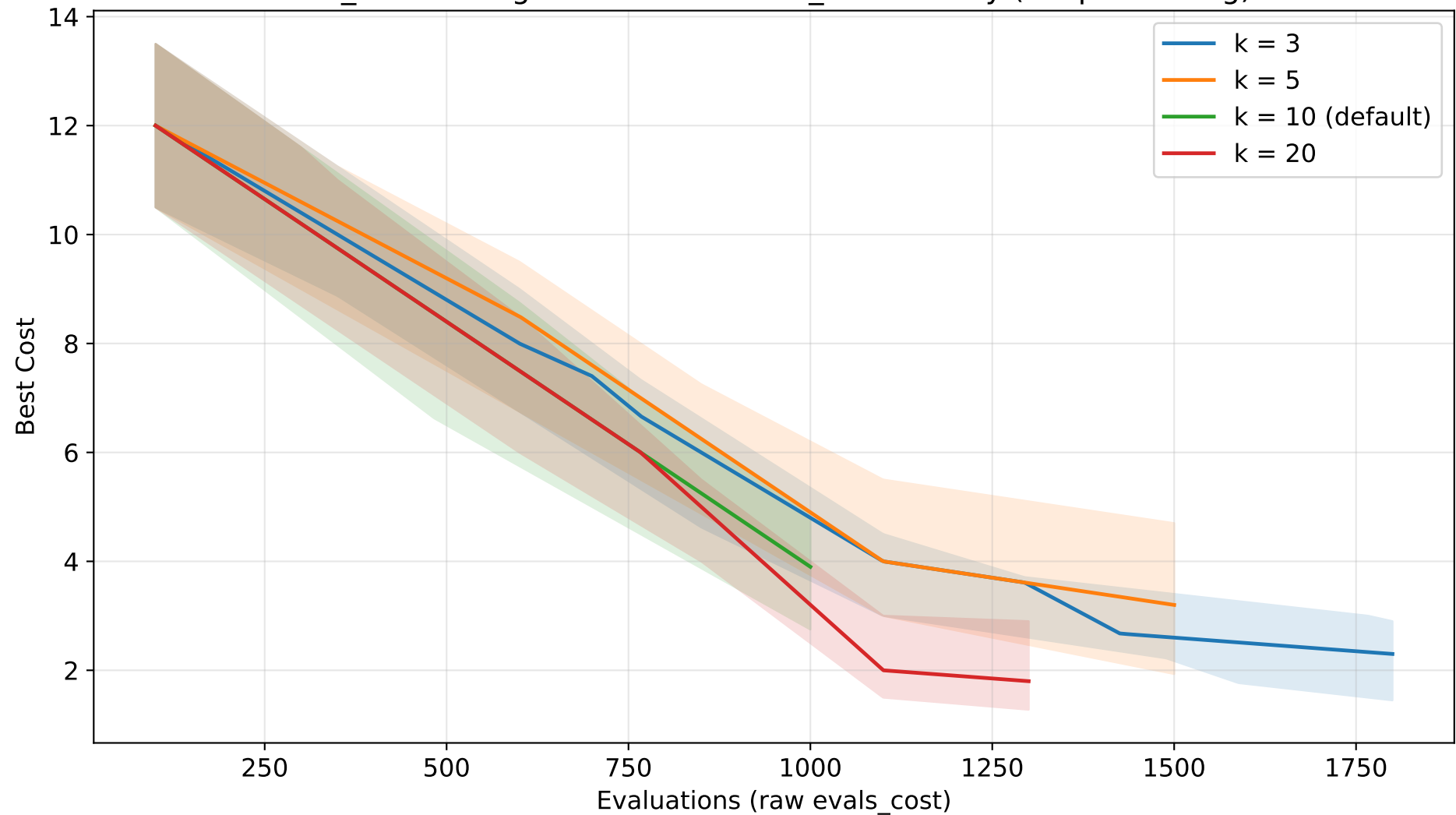
GA_GC convergence - tournament_k sensitivity (GraphColoring)
