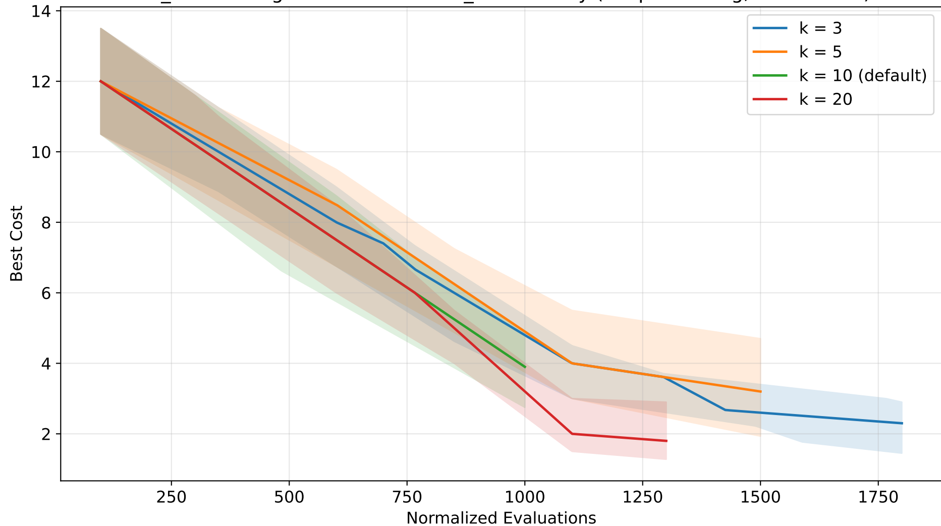
GA_GC convergence - tournament_k sensitivity (GraphColoring, normalized)
