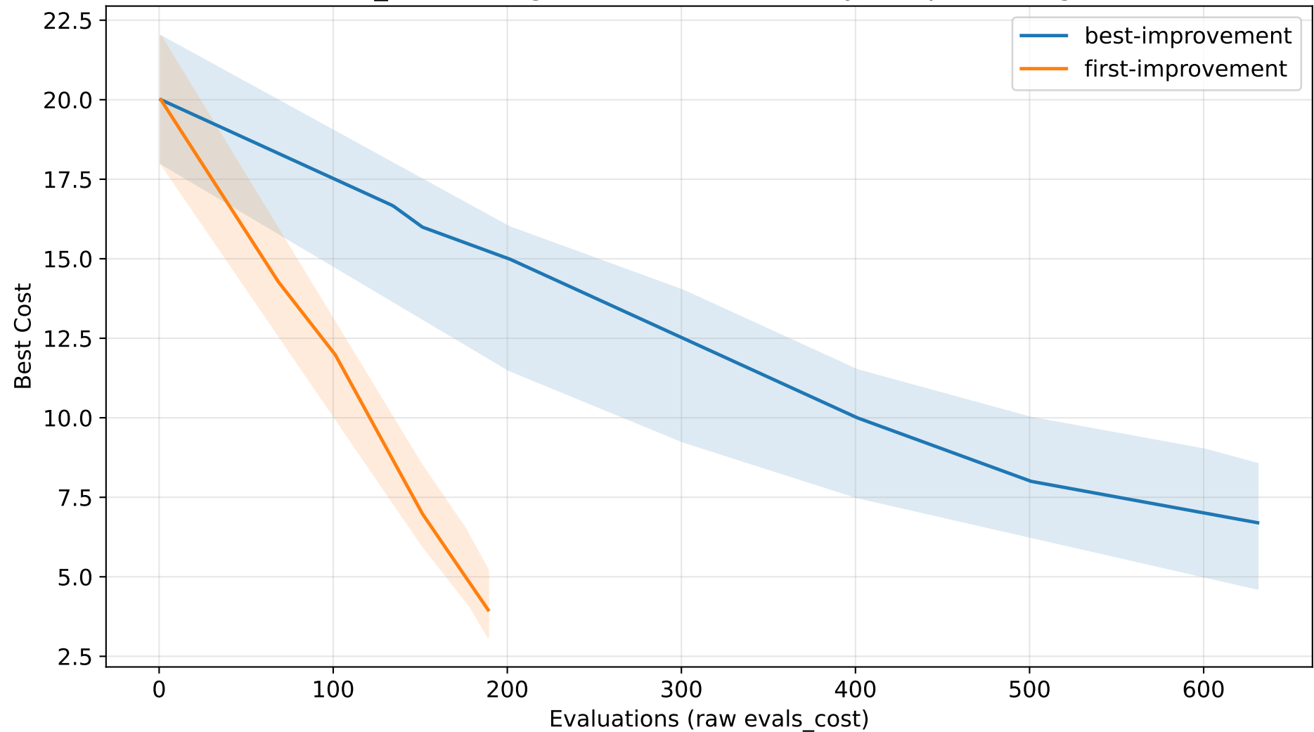
HC_GC convergence - mode sensitivity (GraphColoring)
