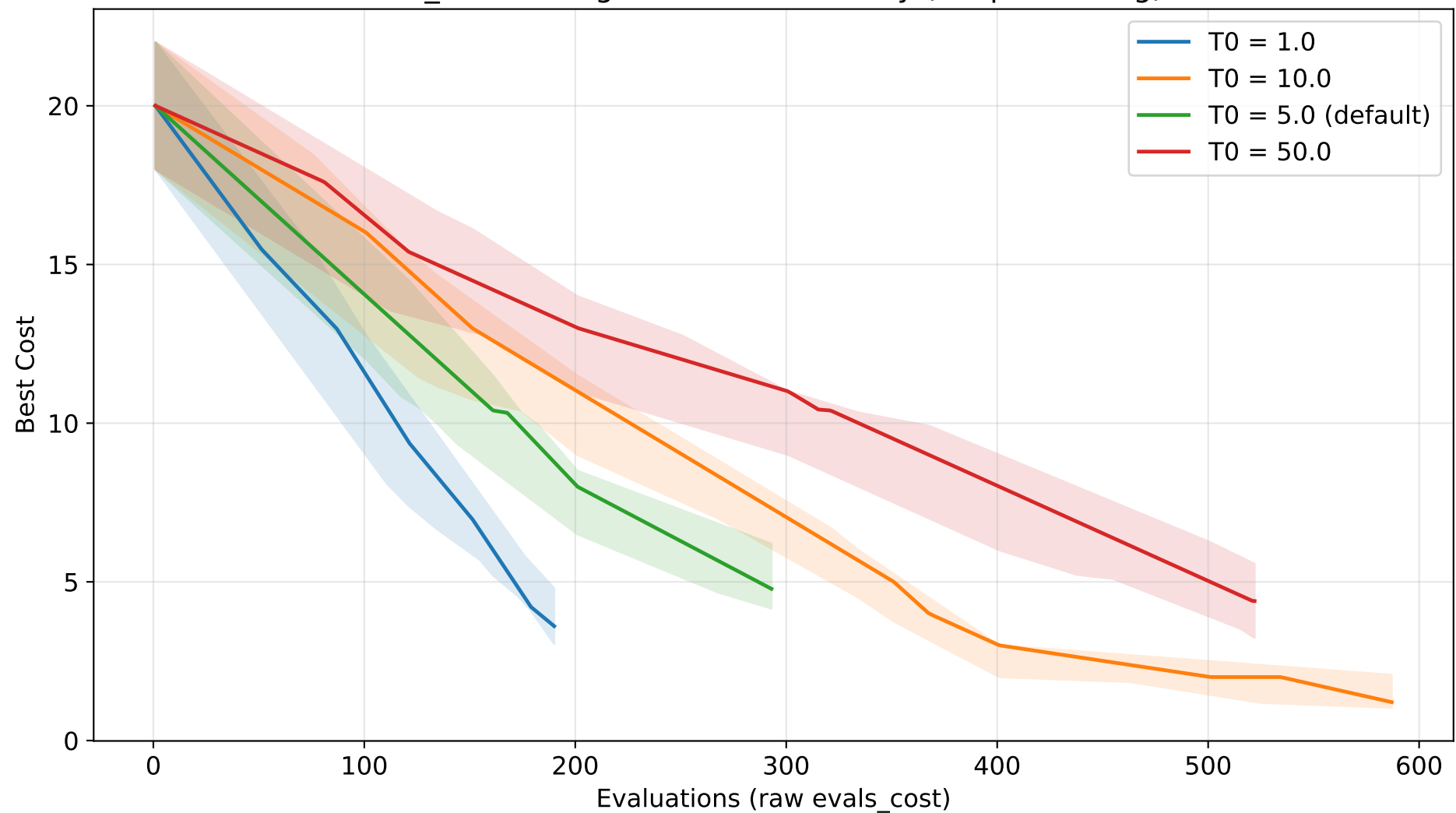
SA_GC convergence - T0 sensitivity (GraphColoring)
