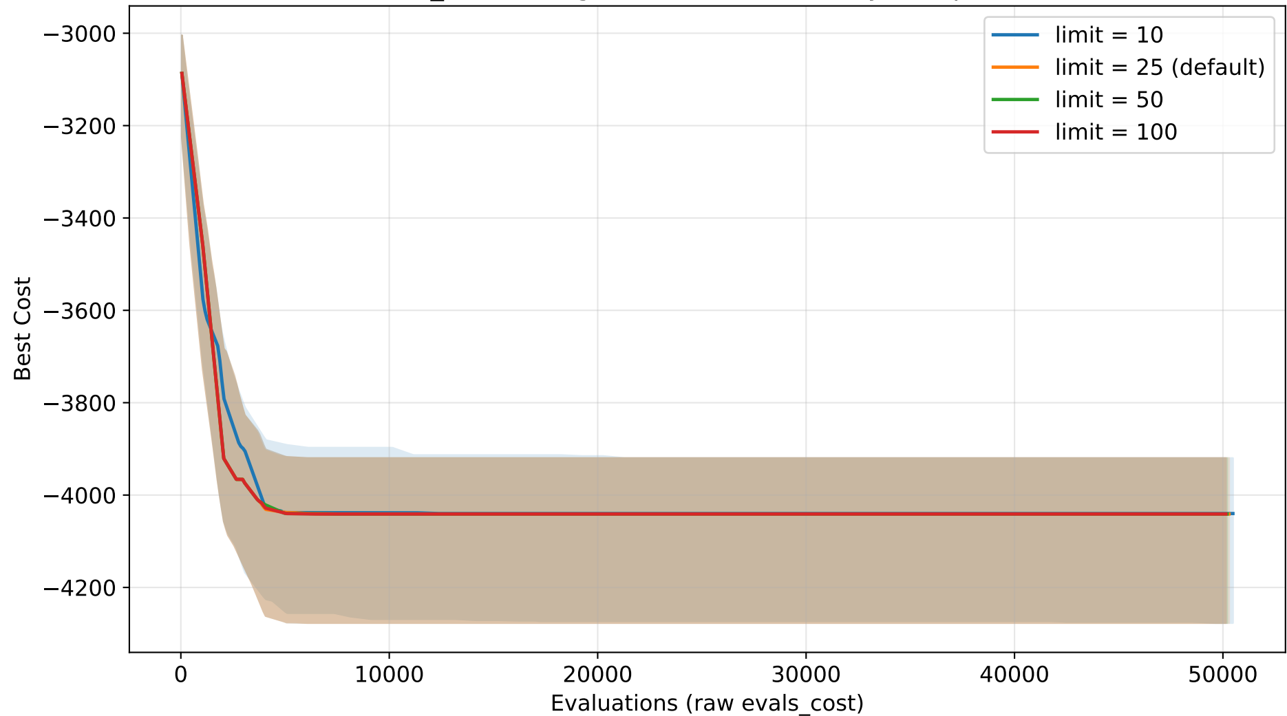
ABC_KP convergence - limit sensitivity (Knapsack)
