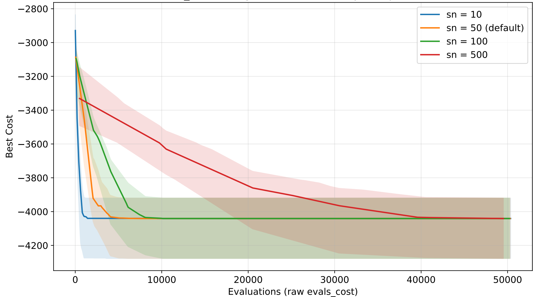
ABC_KP convergence - sn sensitivity (Knapsack)
