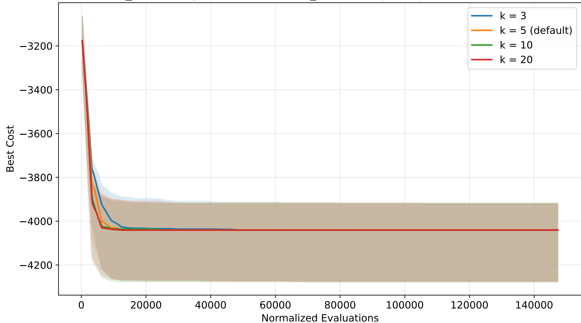
GA_KP convergence - tournament_k sensitivity (Knapsack, normalized)
