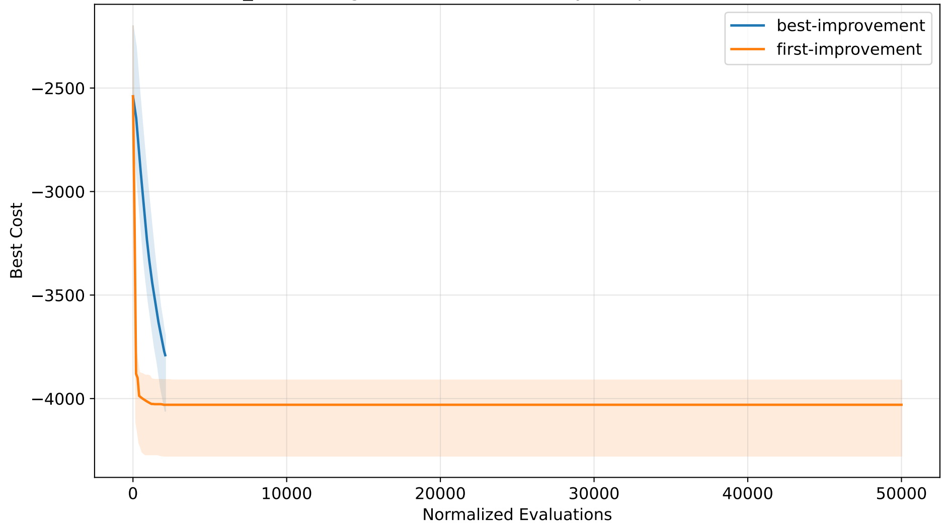
HC_KP convergence - mode sensitivity (Knapsack, normalized)
