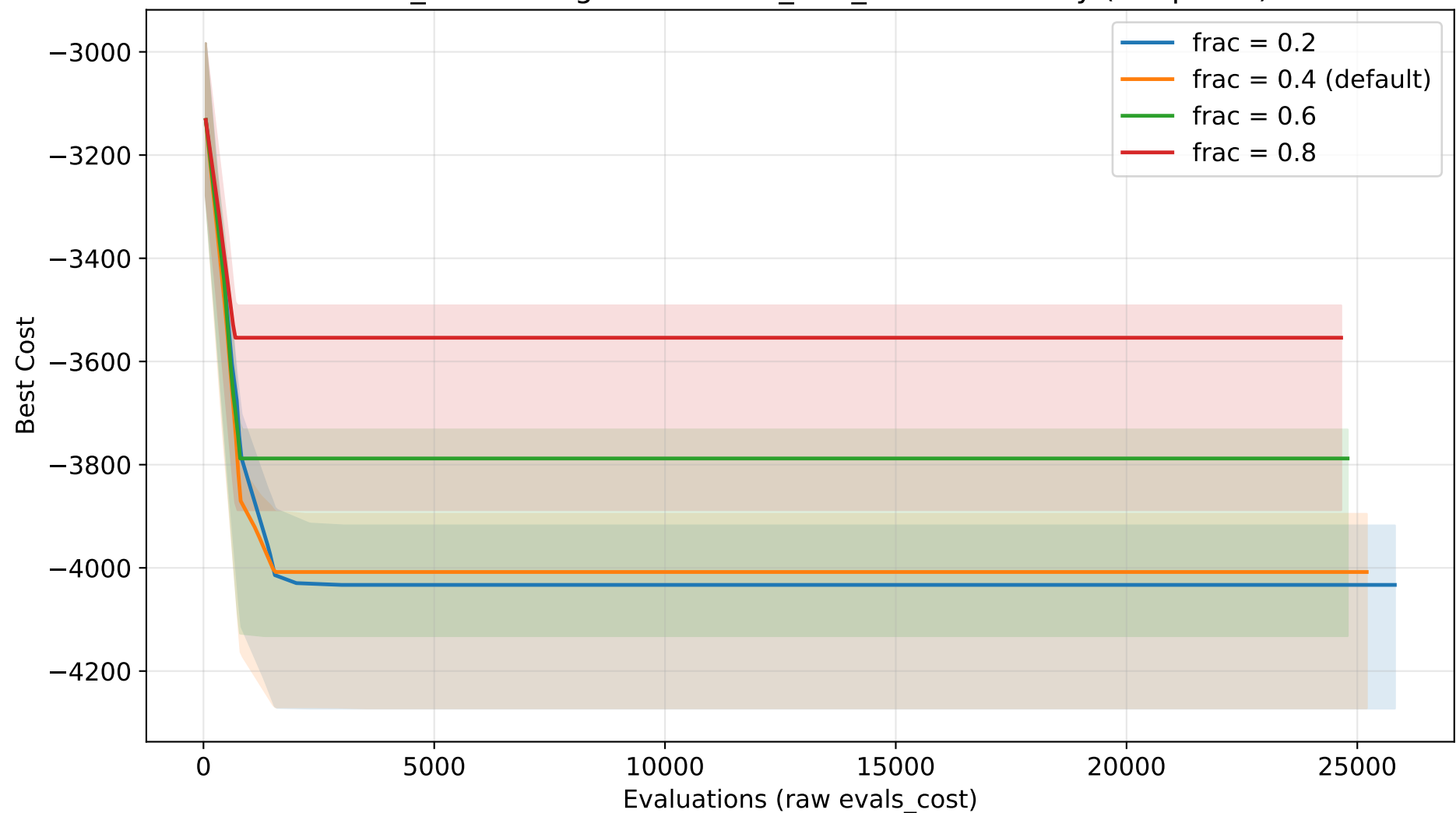
TLBO_KP convergence - move_frac_max sensitivity (Knapsack)
