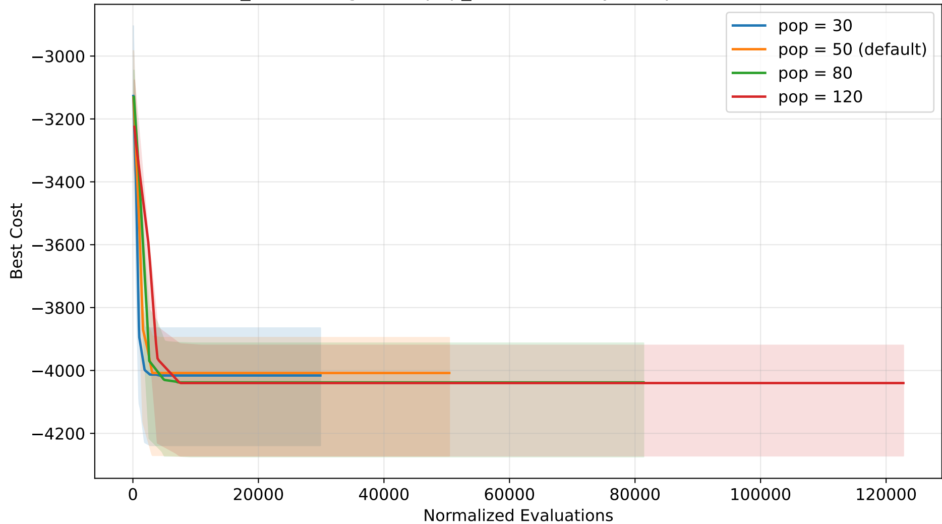
TLBO_KP convergence - pop_size sensitivity (Knapsack, normalized)
