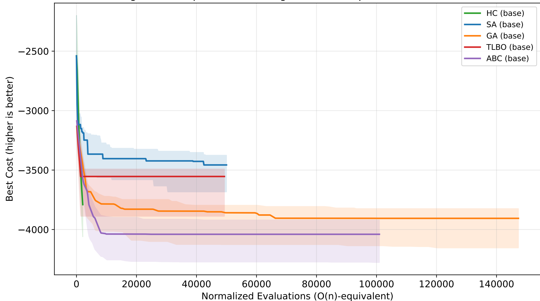
Convergence Comparison — All Algorithms (Knapsack n=100, normalized)
