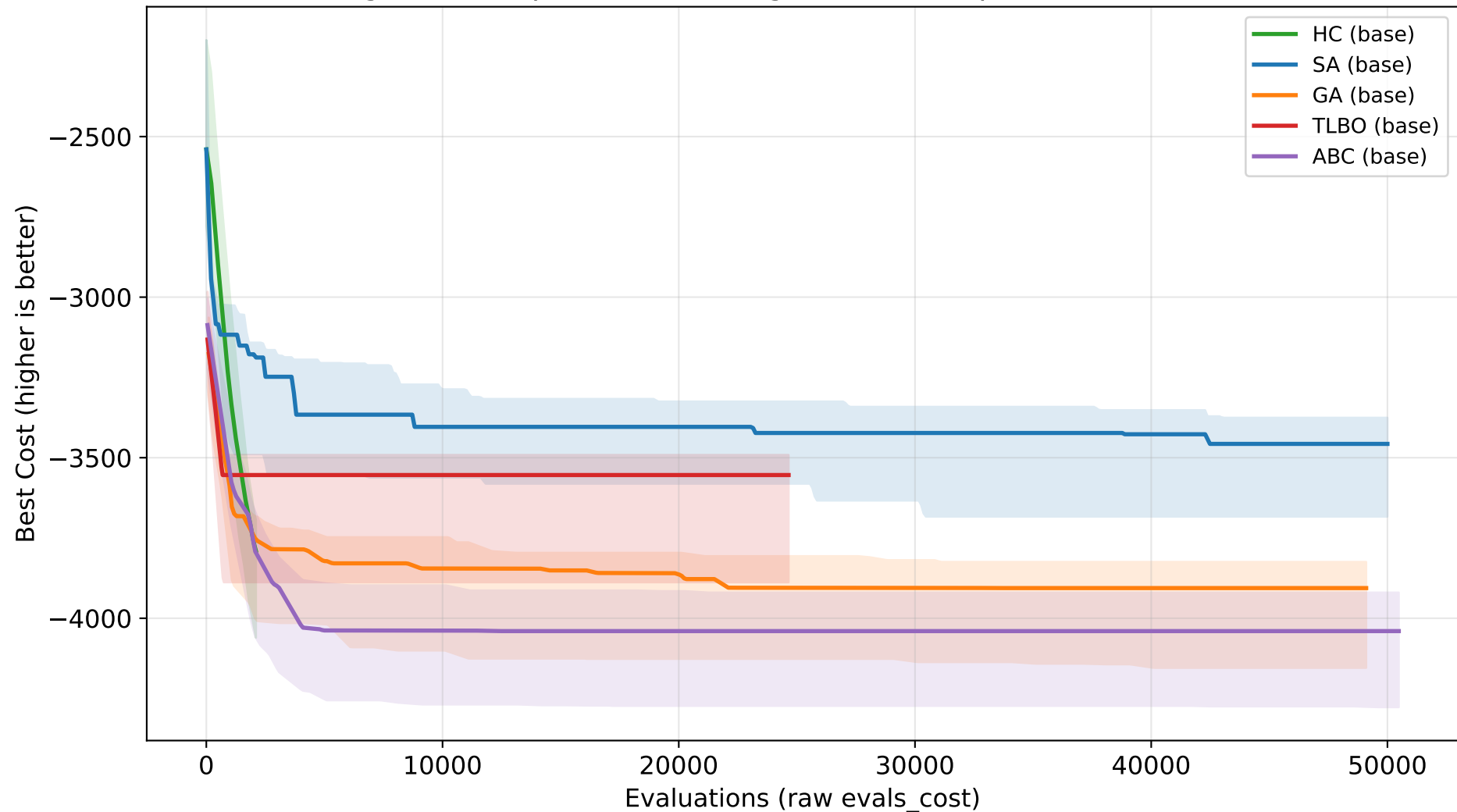
Convergence Comparison — All Algorithms (Knapsack n=100, raw evals)
