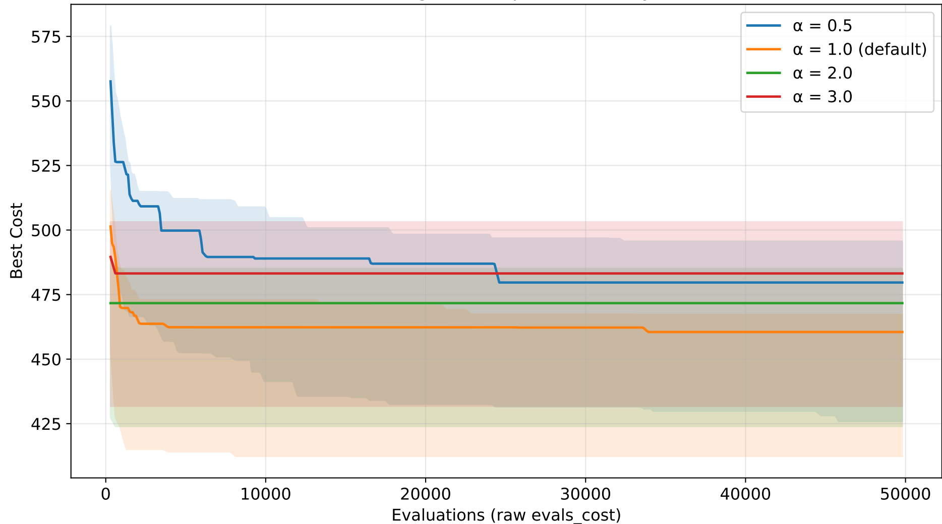
ACO convergence - alpha sensitivity (TSP)
