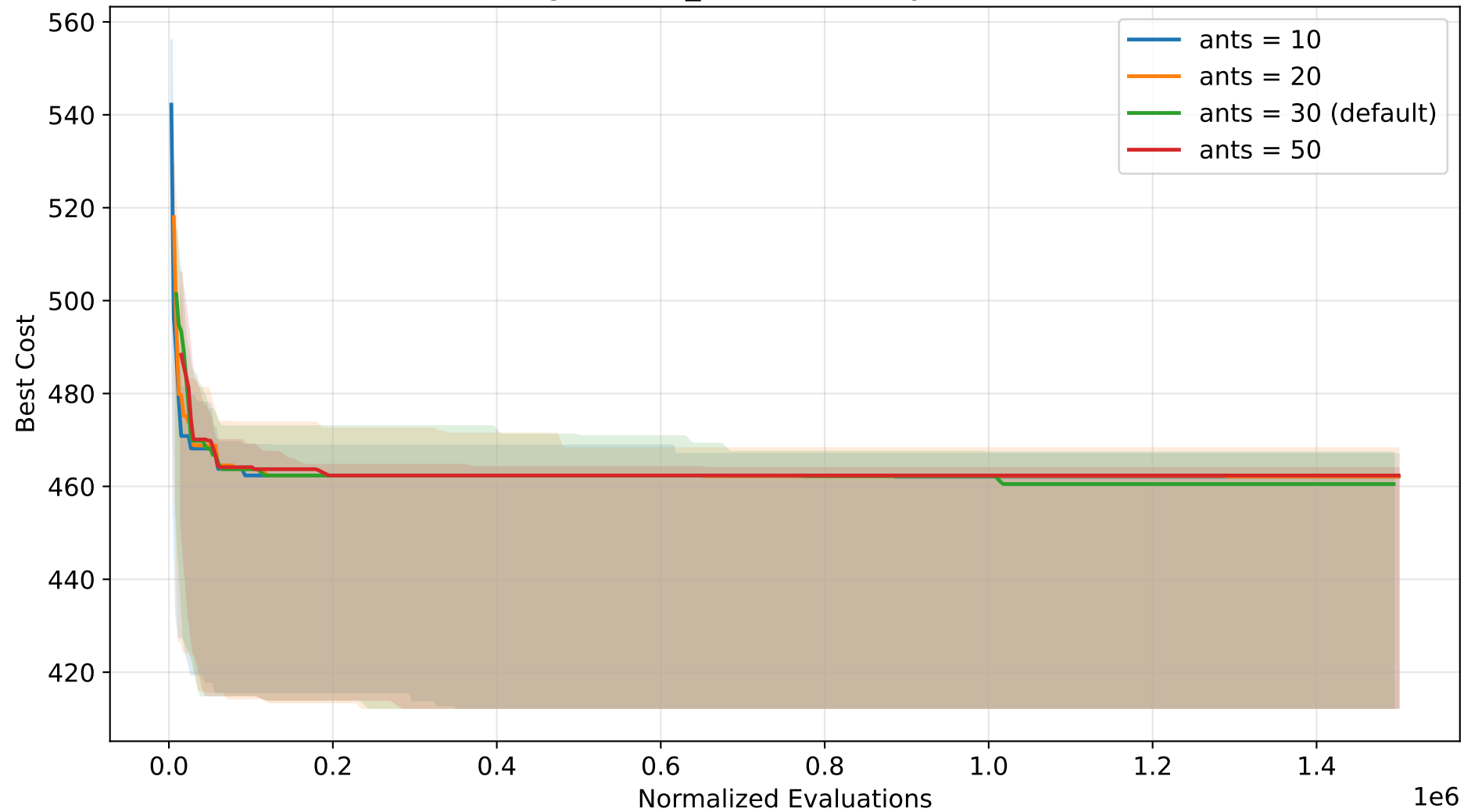
ACO convergence - n_ants sensitivity (TSP, normalized)
