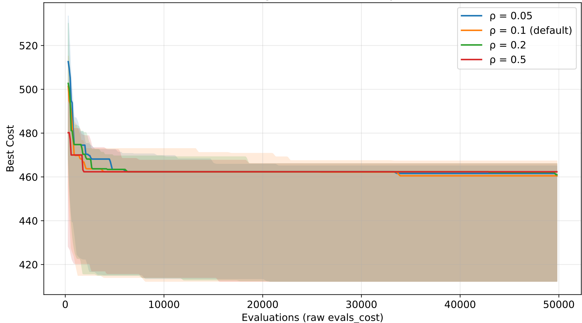
ACO convergence - rho sensitivity (TSP)
