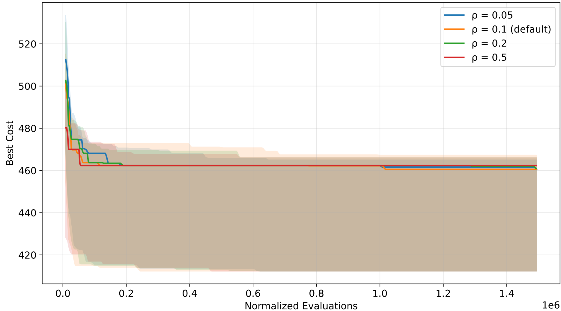
ACO convergence - rho sensitivity (TSP, normalized)
