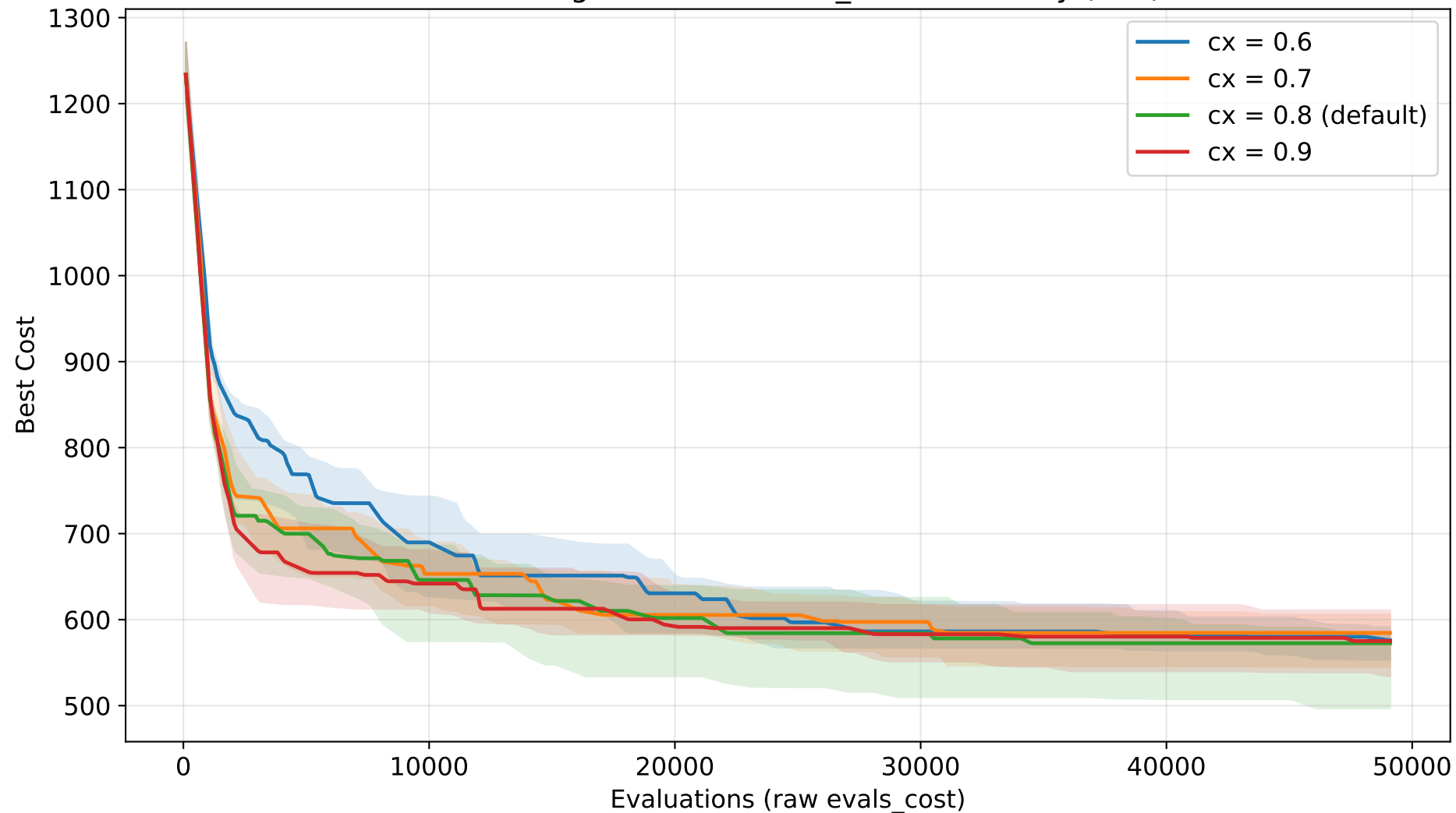
GA convergence - crossover_rate sensitivity (TSP)
