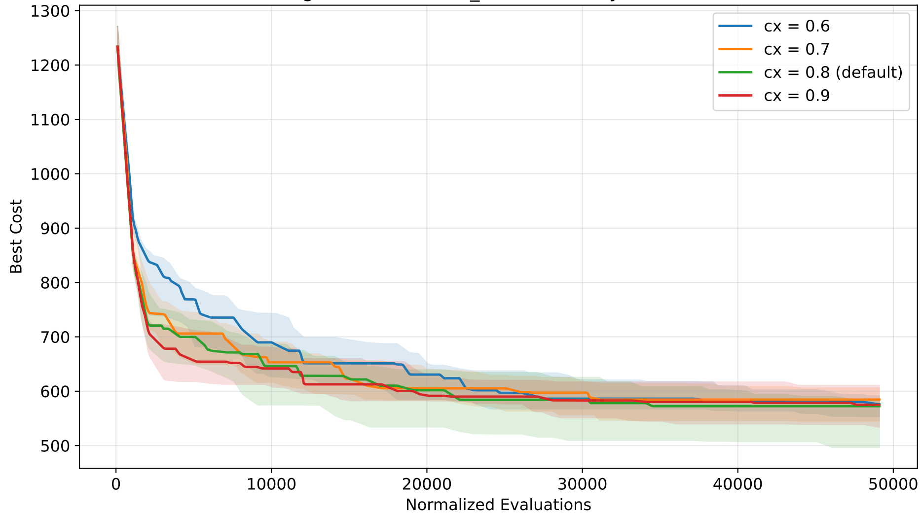
GA convergence - crossover_rate sensitivity (TSP, normalized)
