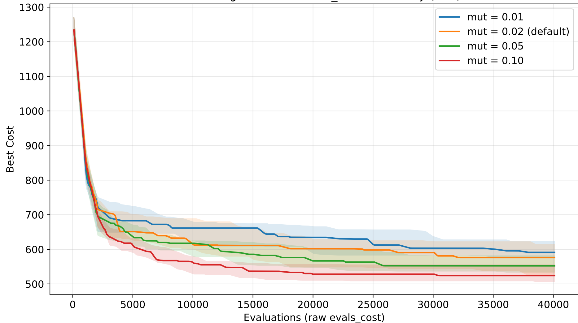
GA convergence - mutation_rate sensitivity (TSP)
