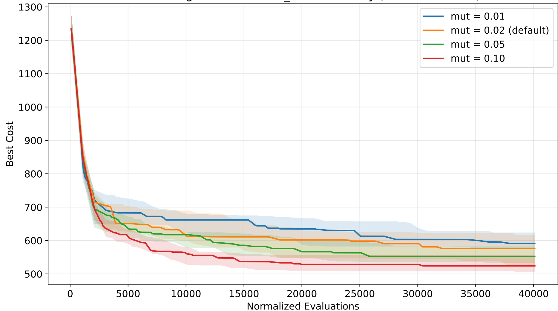
GA convergence - mutation_rate sensitivity (TSP, normalized)
