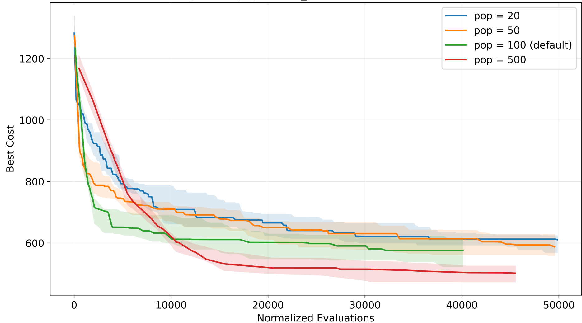
GA convergence - population_size sensitivity (TSP, normalized)
